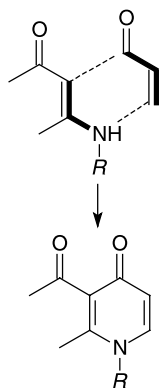
Fig. 1. Regiochemistry of formal aza-[3 + 3] cycloaddition of enaminones and a generic \alpha,\beta -unsaturated carbonyl electrophile
