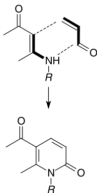
Fig. 1. Regiochemistry of formal aza-[3 + 3] cycloaddition of enaminones and a generic \alpha,\beta -unsaturated carbonyl electrophile
